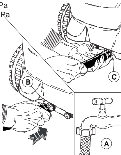
Raccordement hydraulique.
